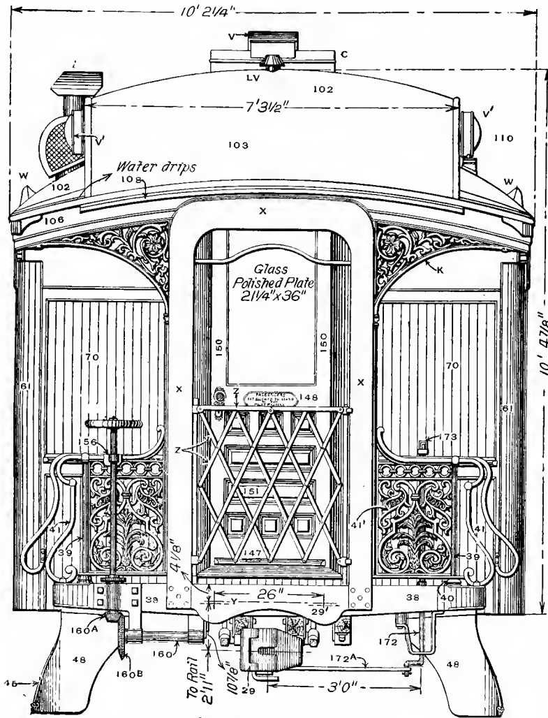
Fig. 539. End Elevation. FIRST-CLASS PASSENGER COACH.
